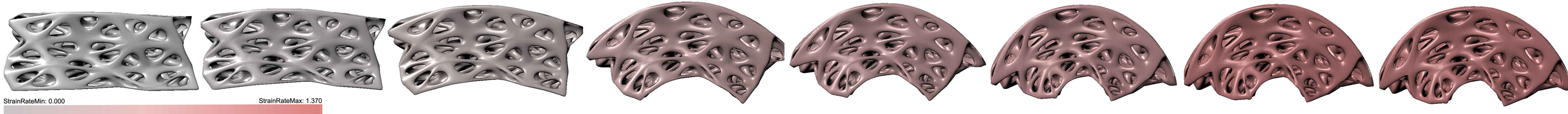
Fig. Deformation Rate: this figure illustrates a representation of the rest position, and shows the seven increasing levels of strain deformation ranging from 0.000 to 1.370.
