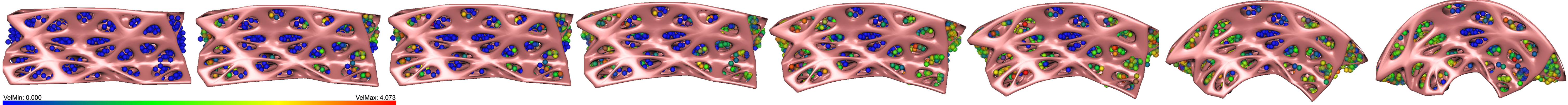
Fig. Flux Velocity: the figure illustrates a fluid particles' velocity during the soft tissues deformation, and shows the diffusion of the fluids within the tissues. In the secondary bone healing process, this flux allows nutrient transportation through cartilages, which influences the healing process significantly.
